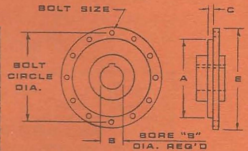
BODY HUB
