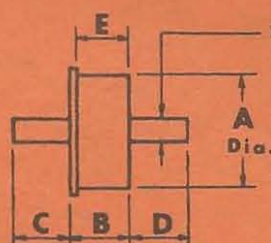
Single Flange Trunnion
