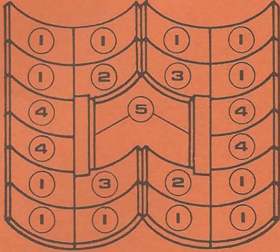
SHELL LINERS
