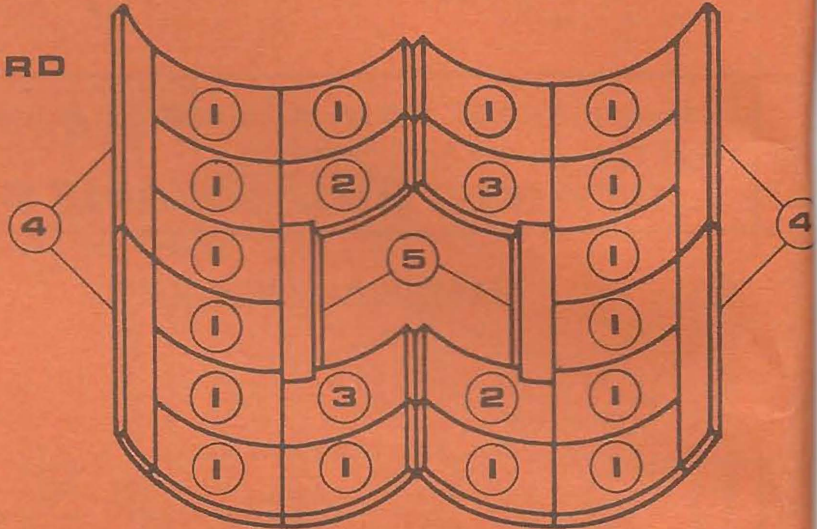
SHELL LINERS
