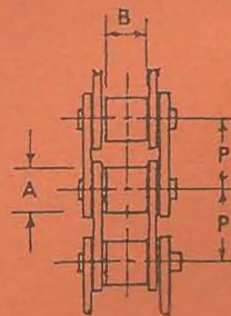
Single Strand
