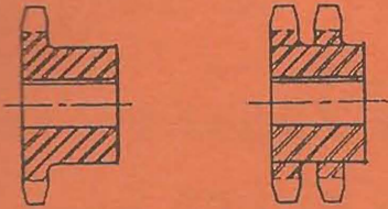
Type "B" Hub - One Side
