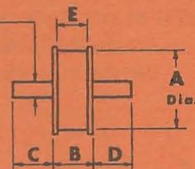
Double Flange Trunnion
