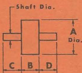
Plain Trunnion
