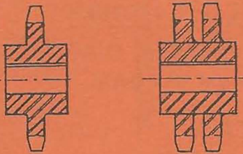
Type "C" Hub - Both Sides
