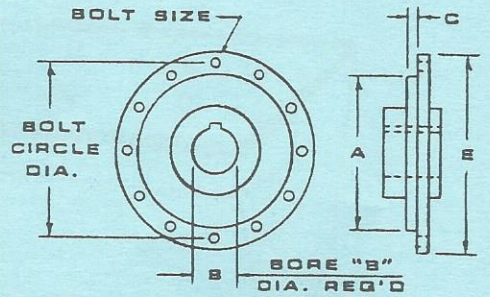
BODY HUB Sprocket/Traction Wheel
