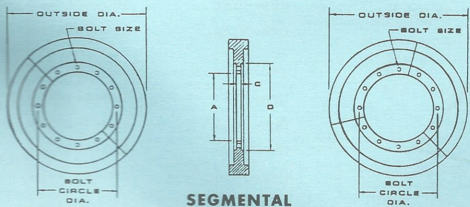
(2) SEGMENTS SEGMENTAL TRACTION WHEELS (3) SEGMENTS
