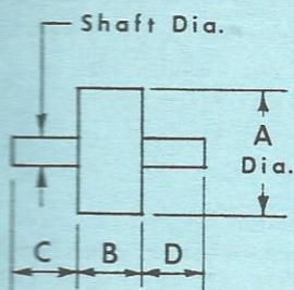
PLAIN TRUNNION (For Gear Drive)
